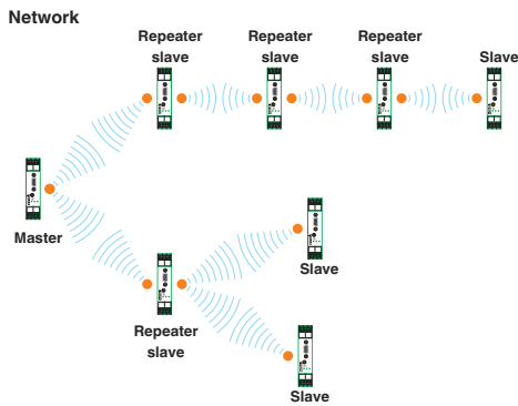
Application drawing
